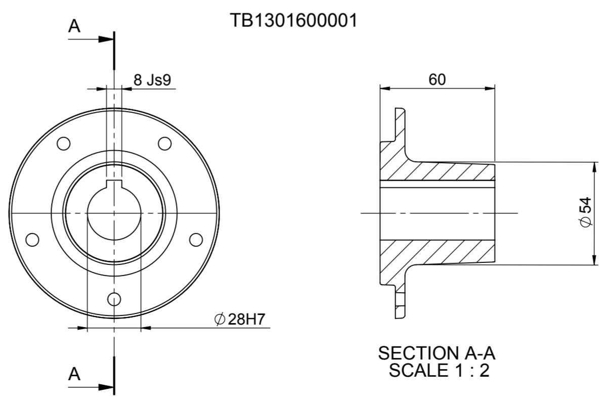
Mounting Details
